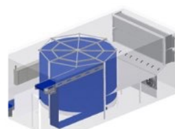
IQF Spiral Freezer
